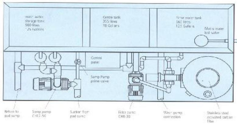
Plan view of HC35 clean system. Covers omitted for clarity. 2400 mm x 1200 mm x 1500 mm high (plus 800 mm clearance required for carbon removal)
